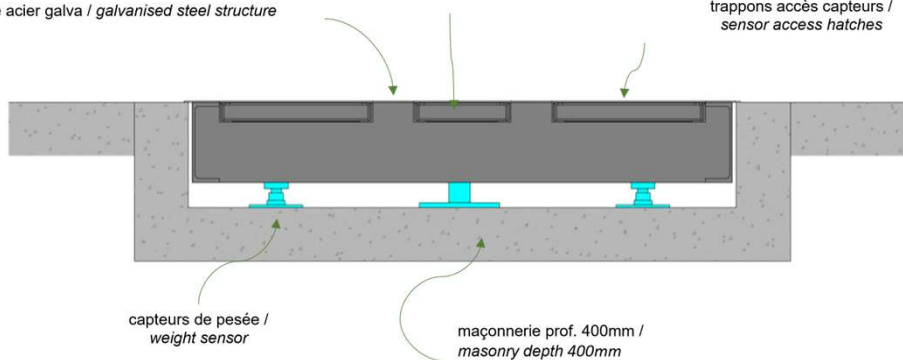
structure acier galva / galvanised steel structure
